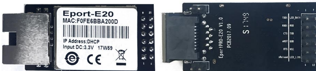
Figure 1. Eport-E20 Appearance
