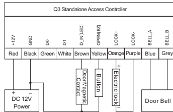
Wiring Diagram (DC Power Supply)
