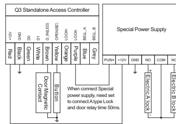
Wiring Diagram (Special Power Supply)
